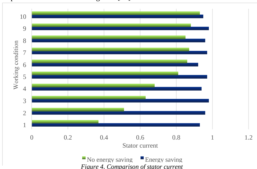
Figure 4. Comparison of stator current
