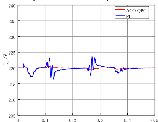
Figure 10: Variation of effective value of u_{CL} when u_G fluctuates.
