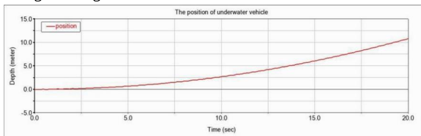
Figure 7: The relationship between the position of AUV's center of mass and time when AUV descent.
