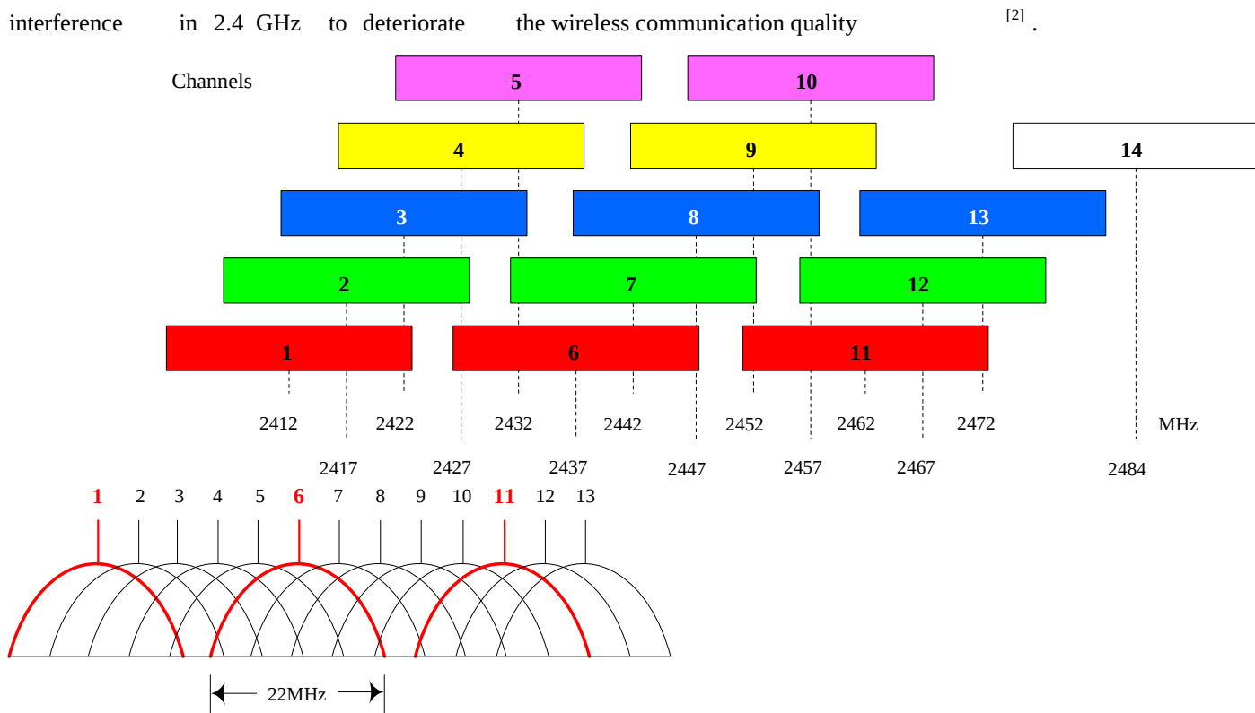
Figure 1: Channel planning of 2.4GHz spectrum
